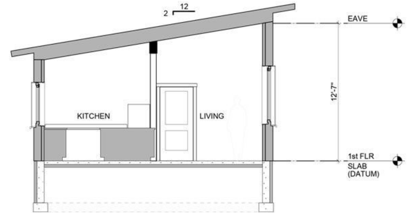
SECTION AT LIVING ROOM
