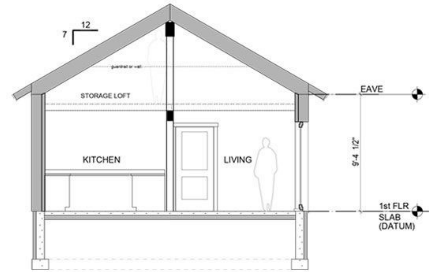
SECTION AT LIVING ROOM
