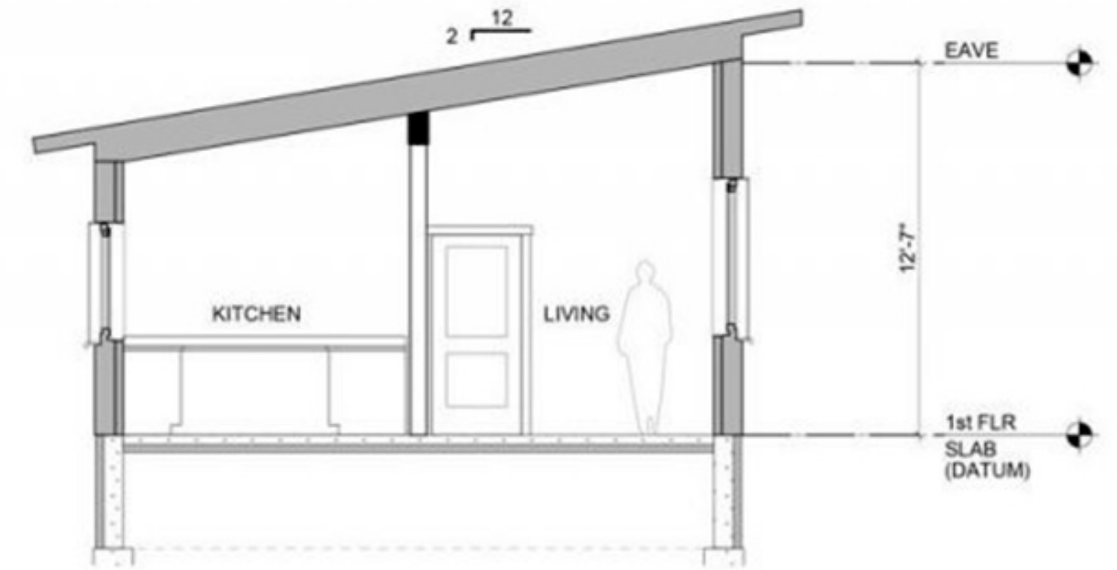
SECTION AT LIVING ROOM
