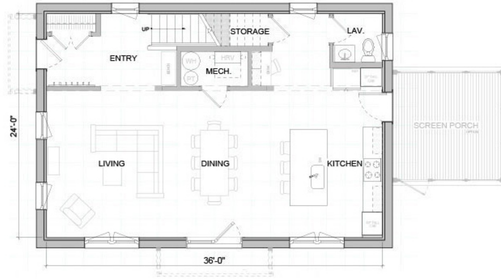
FIRST FLOOR
